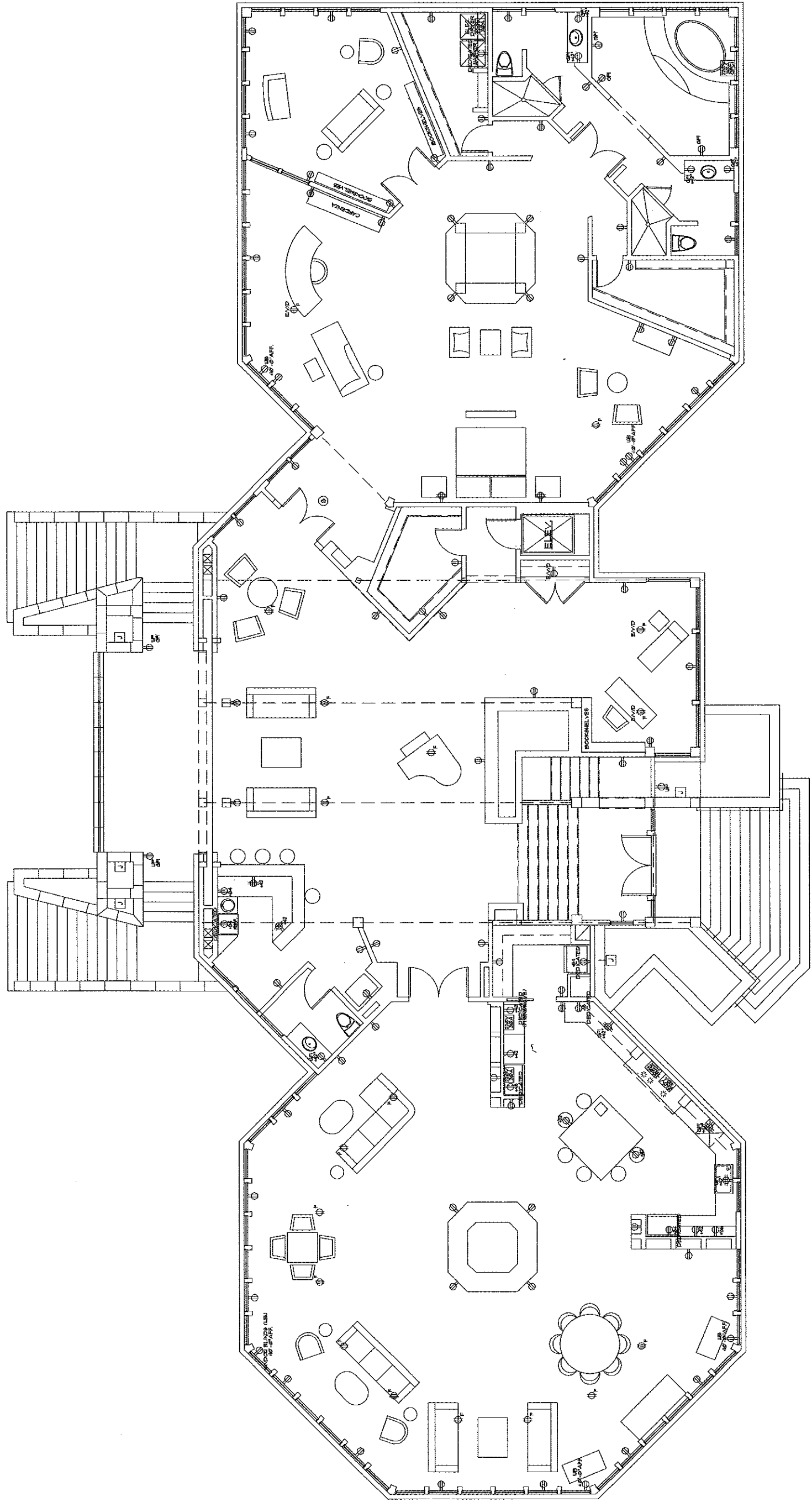
MAIN FLOOR POWER PLAN SCALE: 3/8" = 1'-0" 1/8" = 1'-0" FINISHED
